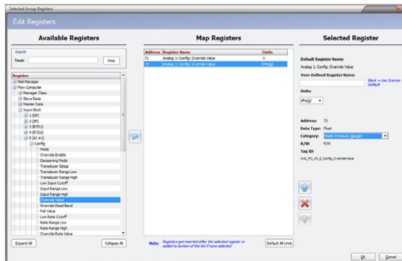
Figure 4.12—Edit Registers screen showing Analog 1 set to output two categories
