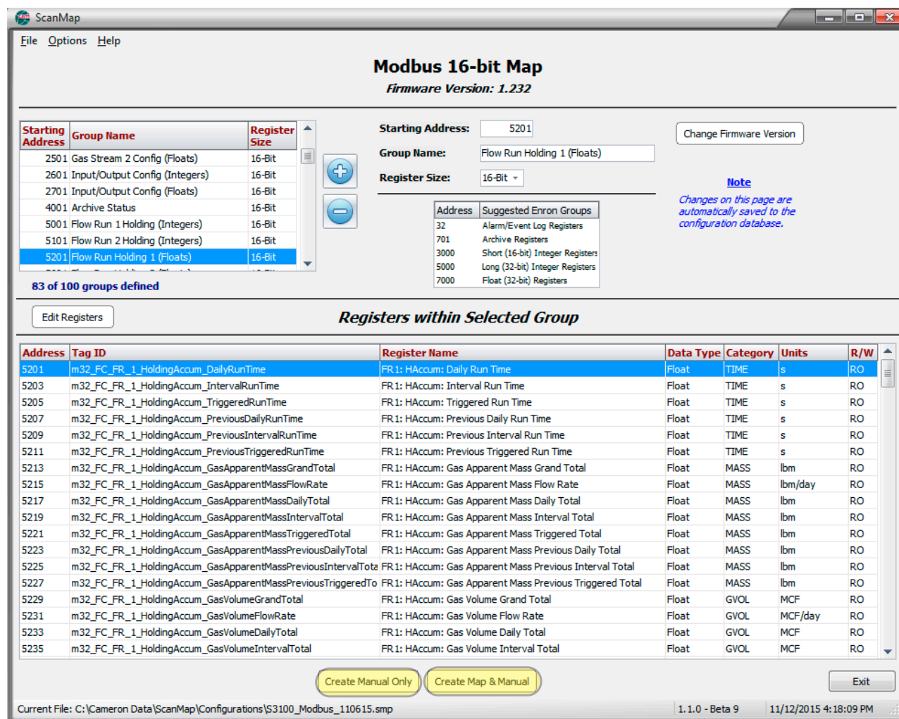
Figure 5.1—Create Manual Only and Create Map and Manual buttons
