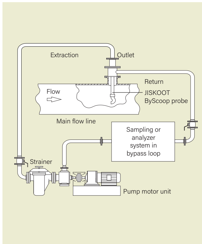
JISKOOT ByScoop probe process diagram
