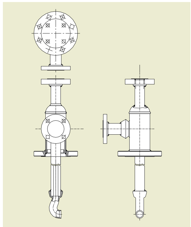
JISKOOT ByScoop sample extraction probe drawing
